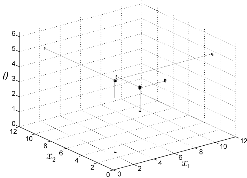
Fig. 4. Solution set in configuration space and its 2D projections
