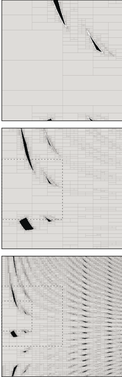
Figure 4: Characterizations of the part of \mathcal{S} in [\mathbf{p}_0] obtained by SIVIA for increasing sizes of [\mathbf{p}_0] ; dotted lines in the bottom two subfigures indicate the correspondence between the frames of the subfigures
