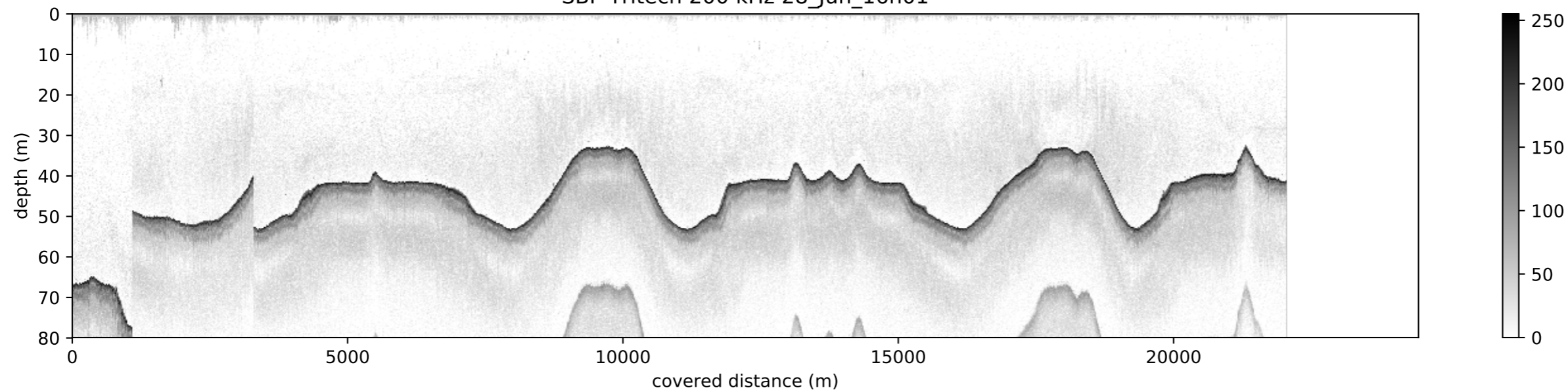
SBP Tritech 200 kHz 28_Jun_16h01
