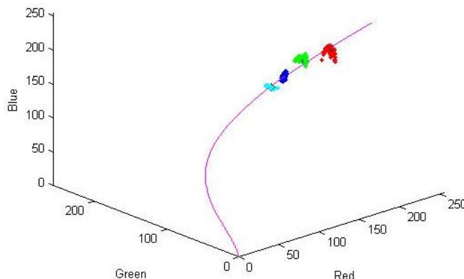
Fig. 2: Initialization pixels at different lengths from Fig.1(b) and the approximated attenuation curve. Each set of pixels of the sub images is color different.
