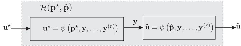
Figure 2. Système \mathcal{H}(\mathbf{p}^*, \hat{\mathbf{p}}) .
