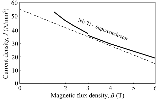
Fig. 3. Critical curve of the superconductor. The true critical curve is in continuous black. The dotted line represents the linear approximation to the previous curve used as quench condition limit in this paper.
