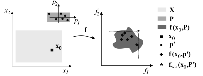
Fig. 2. Worst case scenario approximation of a particular solution \mathbf{x}_0 . The function \mathbf{f} maps \mathbf{x}_0 \in \mathbf{X} and a set of samples \mathbf{P}' \subset \mathbf{P} to objective space. The full image of \mathbf{x}_0 is the region in the objective space marked in dark gray. Note that the worst case is an approximation because it depends on the number of the samples n_s and their spreading quality; if n_s \rightarrow \infty , \mathbf{P}' \rightarrow \mathbf{P} .
