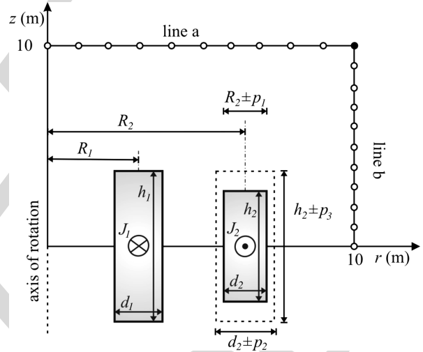
Fig. 1. Robust configuration of the TEAM 22 problem. The parameters R_1 , d_1 and h_1 are known, the design parameters \mathbf{x} = \{R_2, d_2, h_2\} have to be optimized by considering the additive uncertainty parameter \mathbf{p} = \{p_1, p_2, p_3\} that represents the rounding or measurement errors, for instance.
