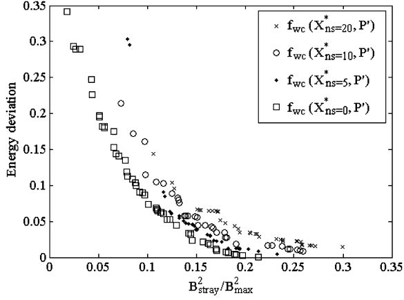
Fig. 4. The dependency of the robust Pareto front on the sample's amount. The smaller n_s caused bad estimation of the individuals' worst case performance, leading their fronts situate quite below of an ideal location.
